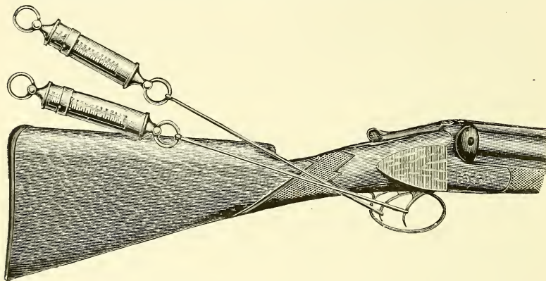
The Correct Angle to Test the Weight of Trigger-Pulls.
